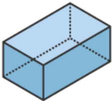
Cuboid
