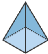
Square-based pyramid
